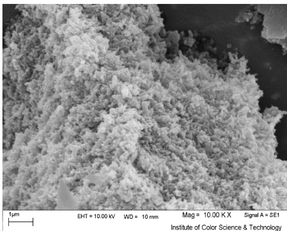
Fig. 3 – SEM image of PANI salt.
